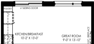
GROUND FLOOR ELEV. C
